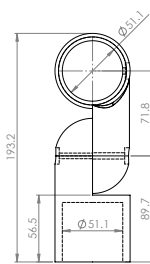
PLAN VIEW
