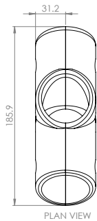
PLAN VIEW
